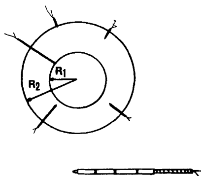
Figure 3. Reactor thermocouple positions.
