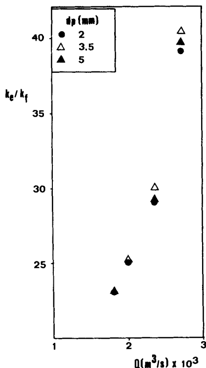
Figure 6. Particle diameter effect on ke/kf .
