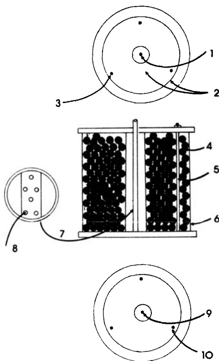
Figure 2. Radial-flow reactor.
