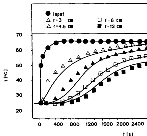
Figure 4. Bed temperature response.
